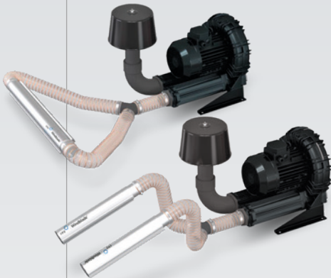
Configuration example for 2 single input blades
