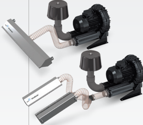
Configuration example for 2 single input blades
