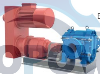
Execution with simple-belt variator drive
