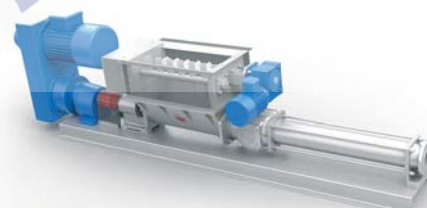
Execution with hopper and infeed screw; with bridge breaker system driven by independent speed reducer.
