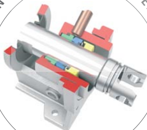
DOUBLE MECHANICAL SEAL
