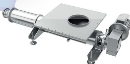
Eccentric screw pump with hopper and special suction cover to be connected to silos
