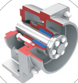
GLAND PACKING
